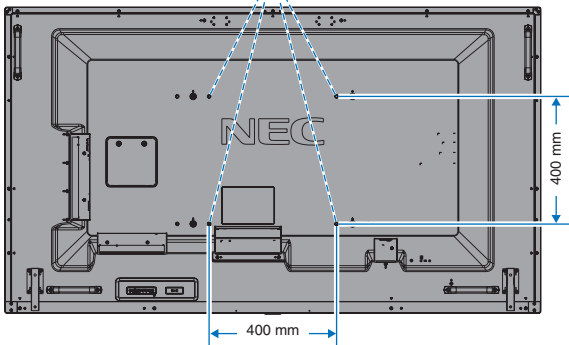
VESA Mounting Interface (M8)
