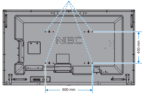
Mounting Interface (M8)
