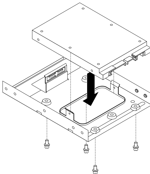
Figure 24. Installing the solid state drive into the adapter
